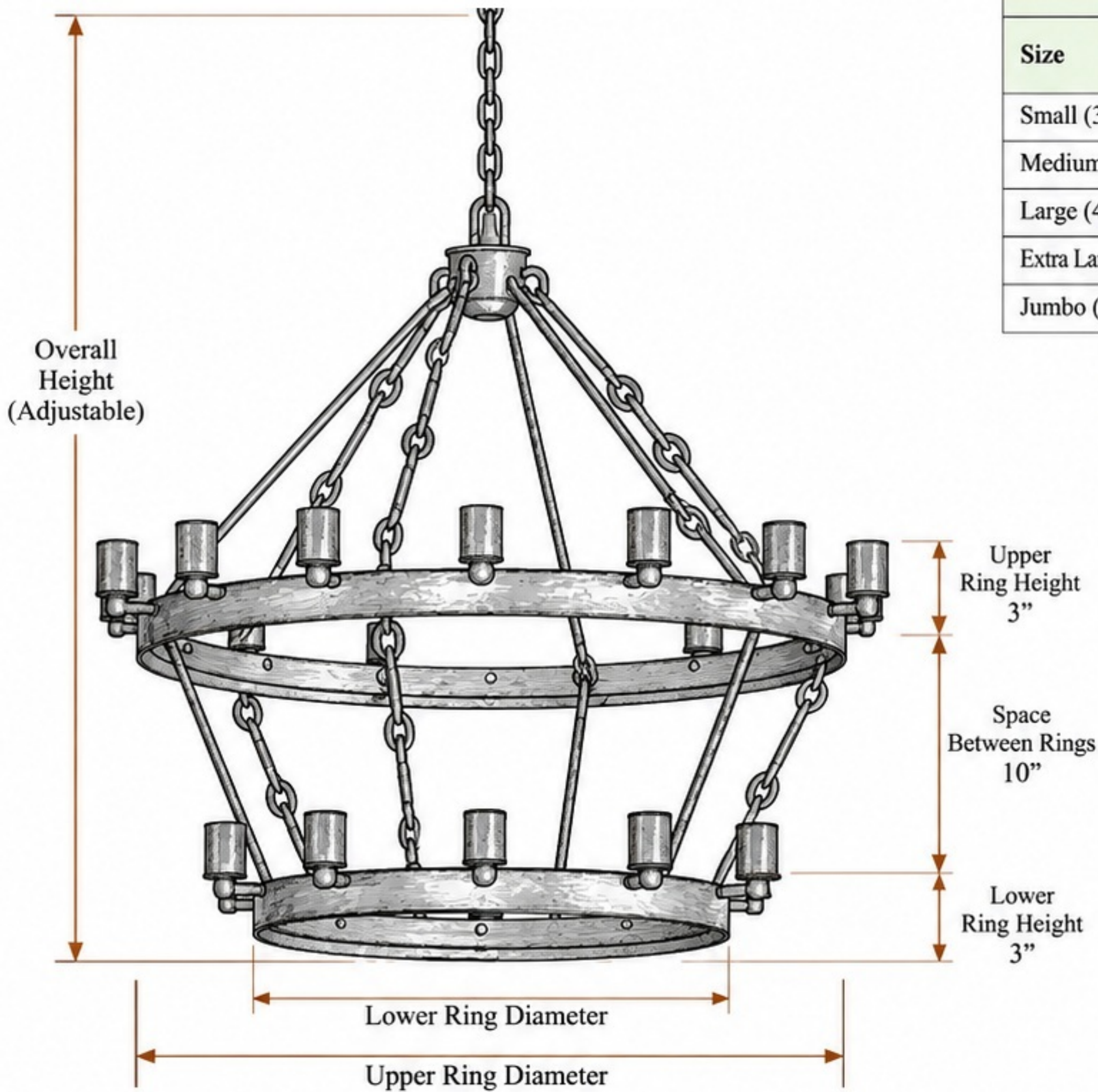
FRONT VIEW
