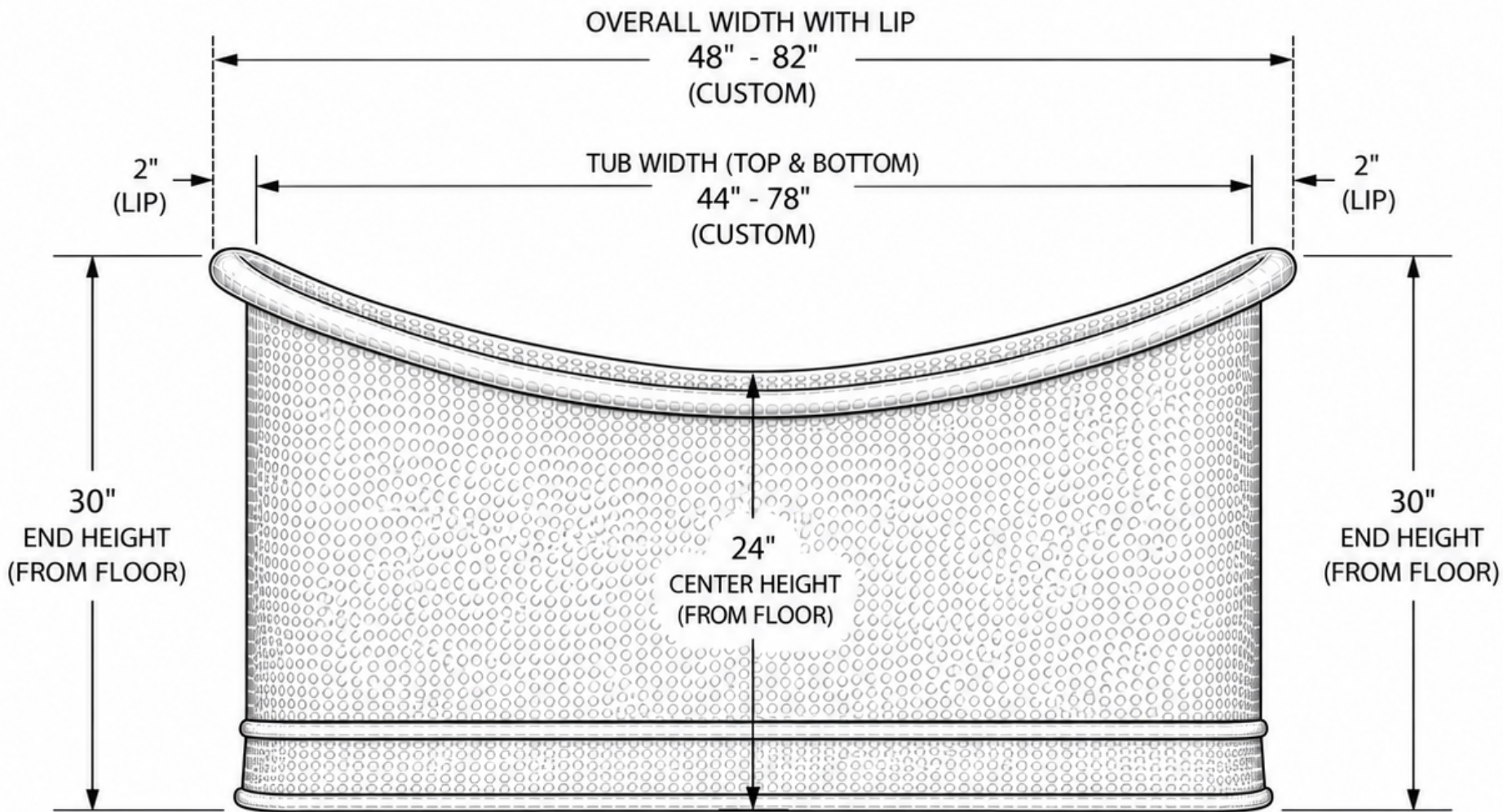
FRONT ELEVATION
