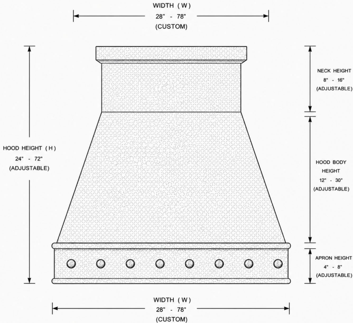
FRONT ELEVATION
