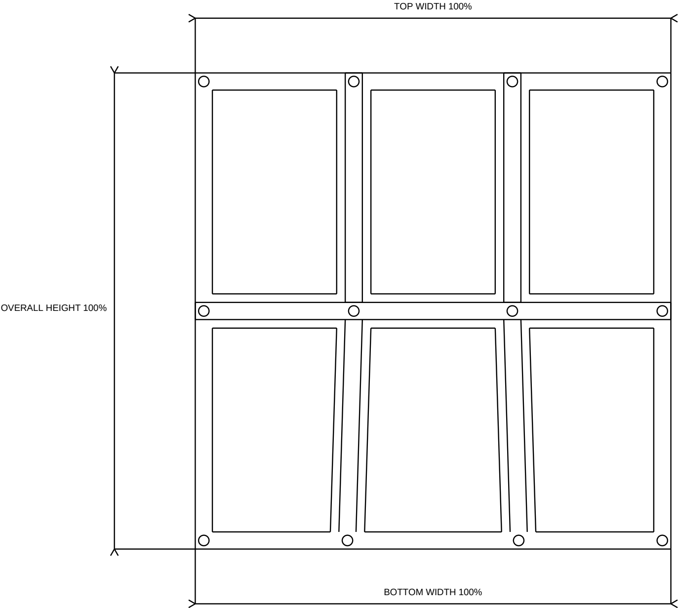
RIVETED THREE-BAY ZINC RANGE HOOD - PROJECTING APRON PROPORTIONAL FRONT ELEVATION - DESIGN INTENT ONLY
