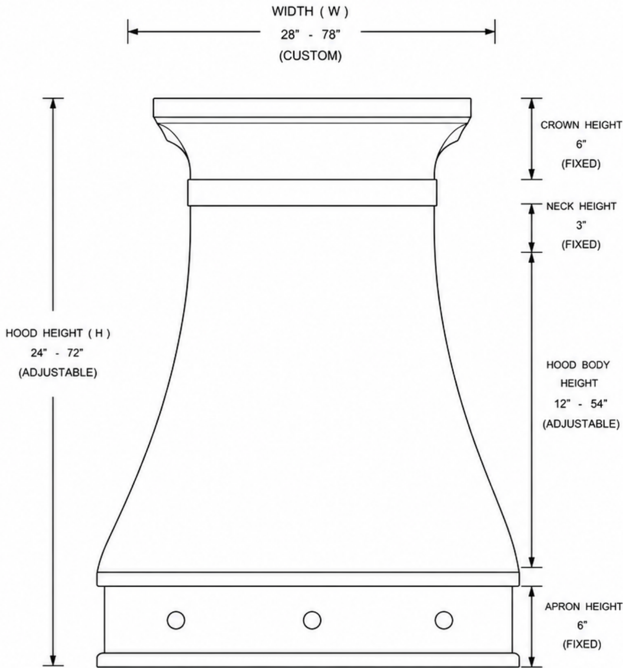
FRONT ELEVATION
