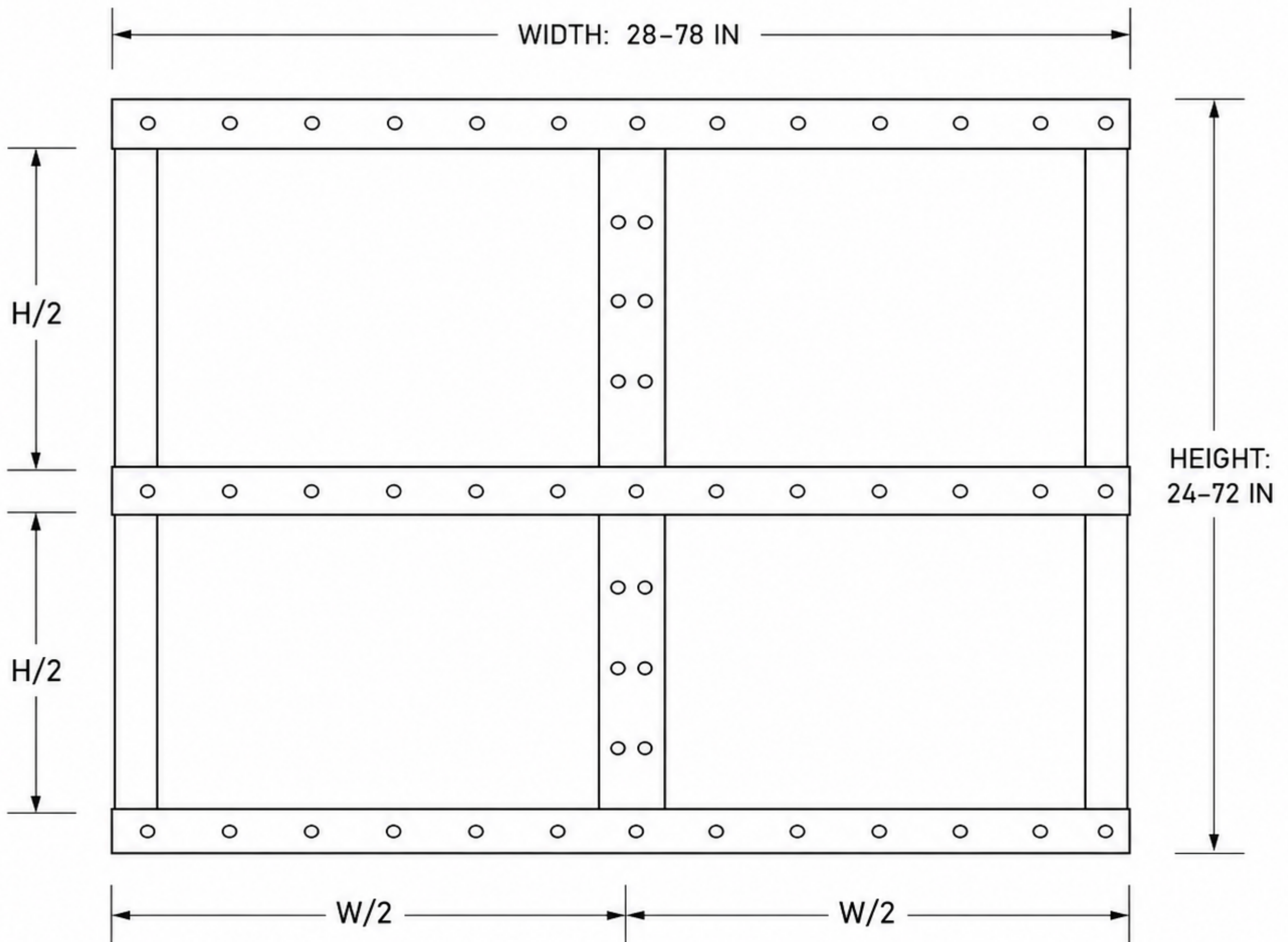
FRONT ELEVATION
