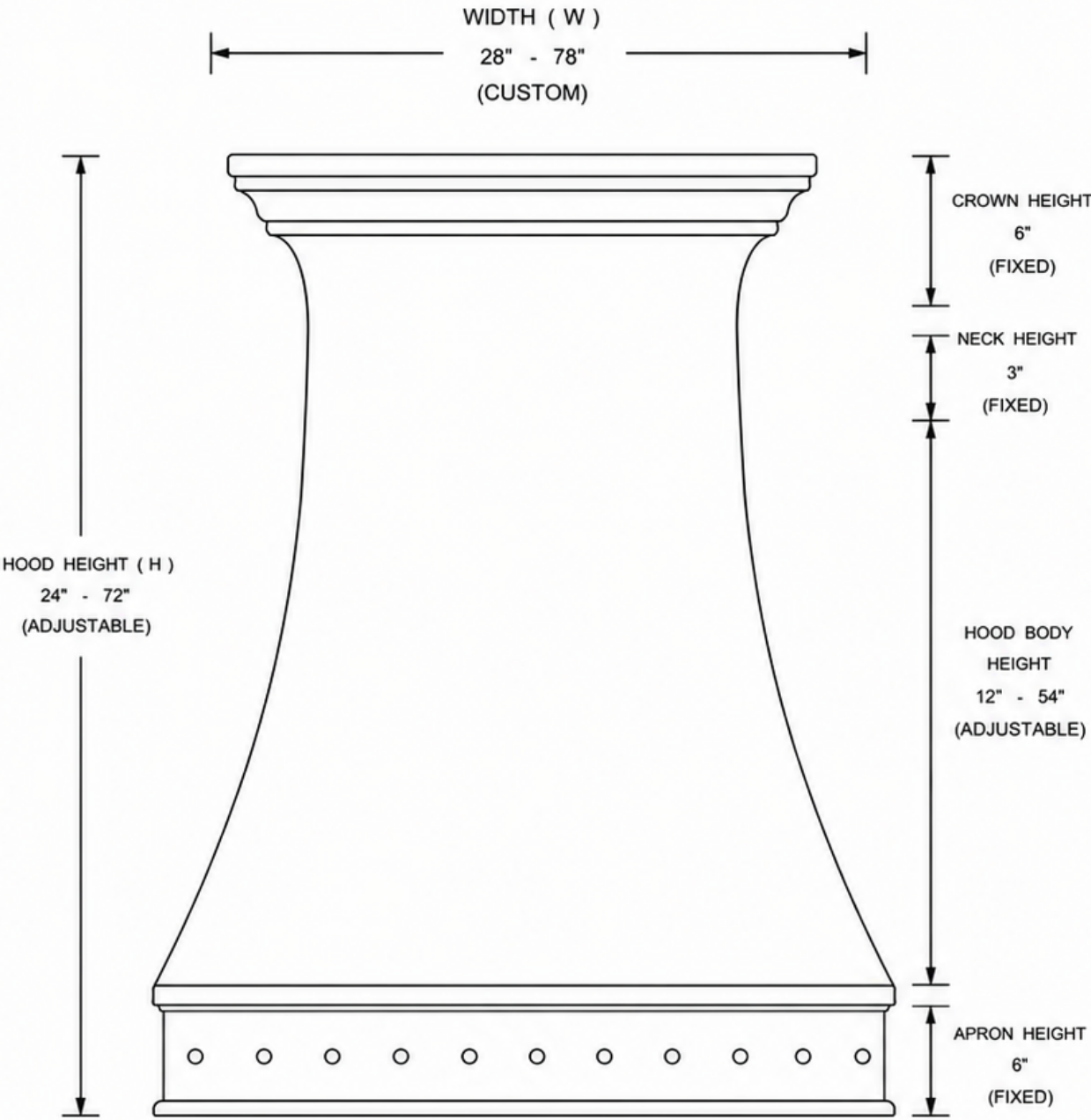
FRONT ELEVATION
