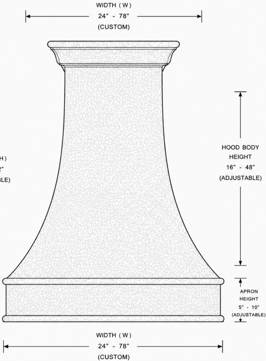
FRONT ELEVATION
