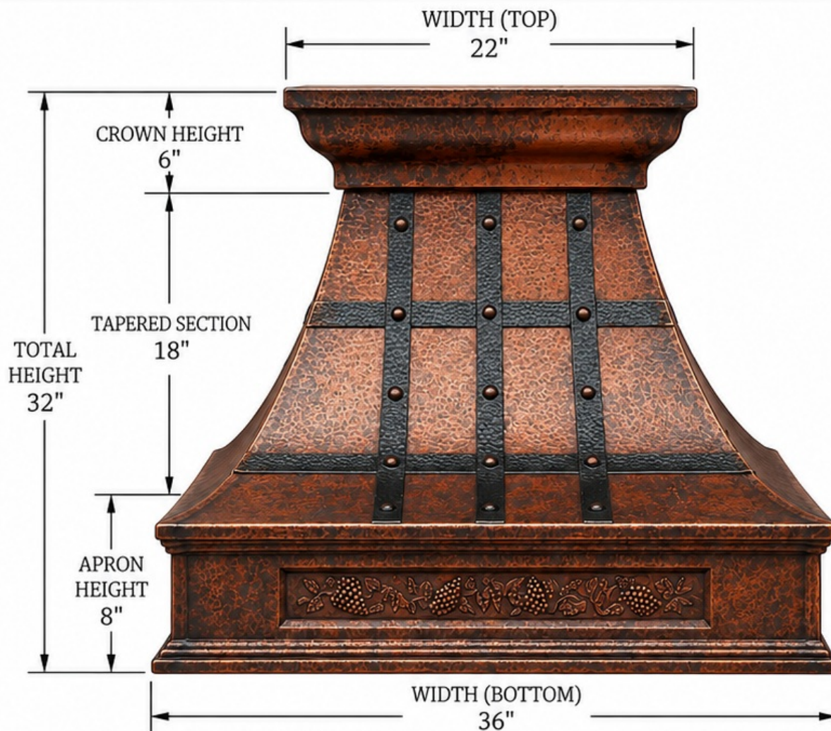
FRONT VIEW
