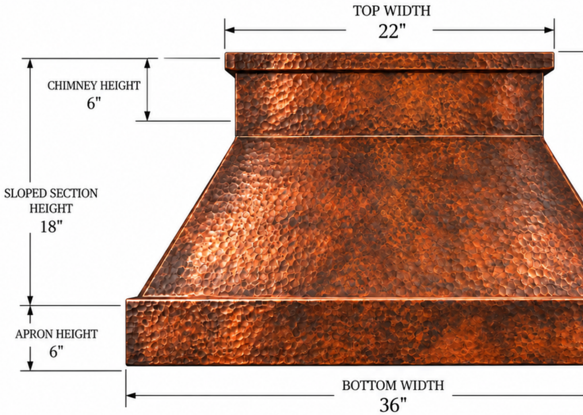
FRONT VIEW
