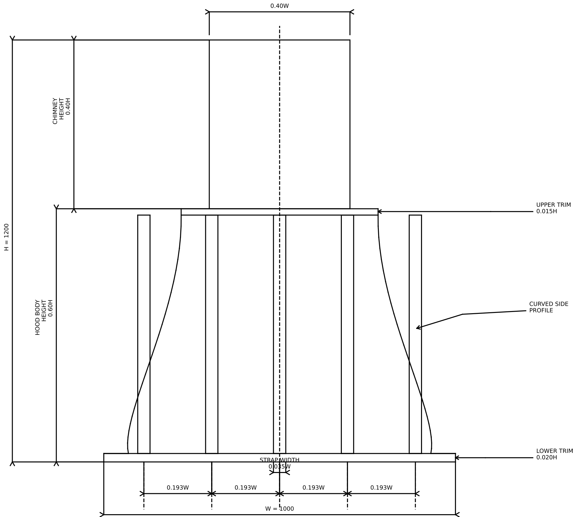
FRONT ELEVATION — WALL-MOUNT RANGE HOOD CENTERED CHIMNEY AND CENTERED STRAP LAYOUT
