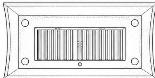
BOTTOM VIEW
