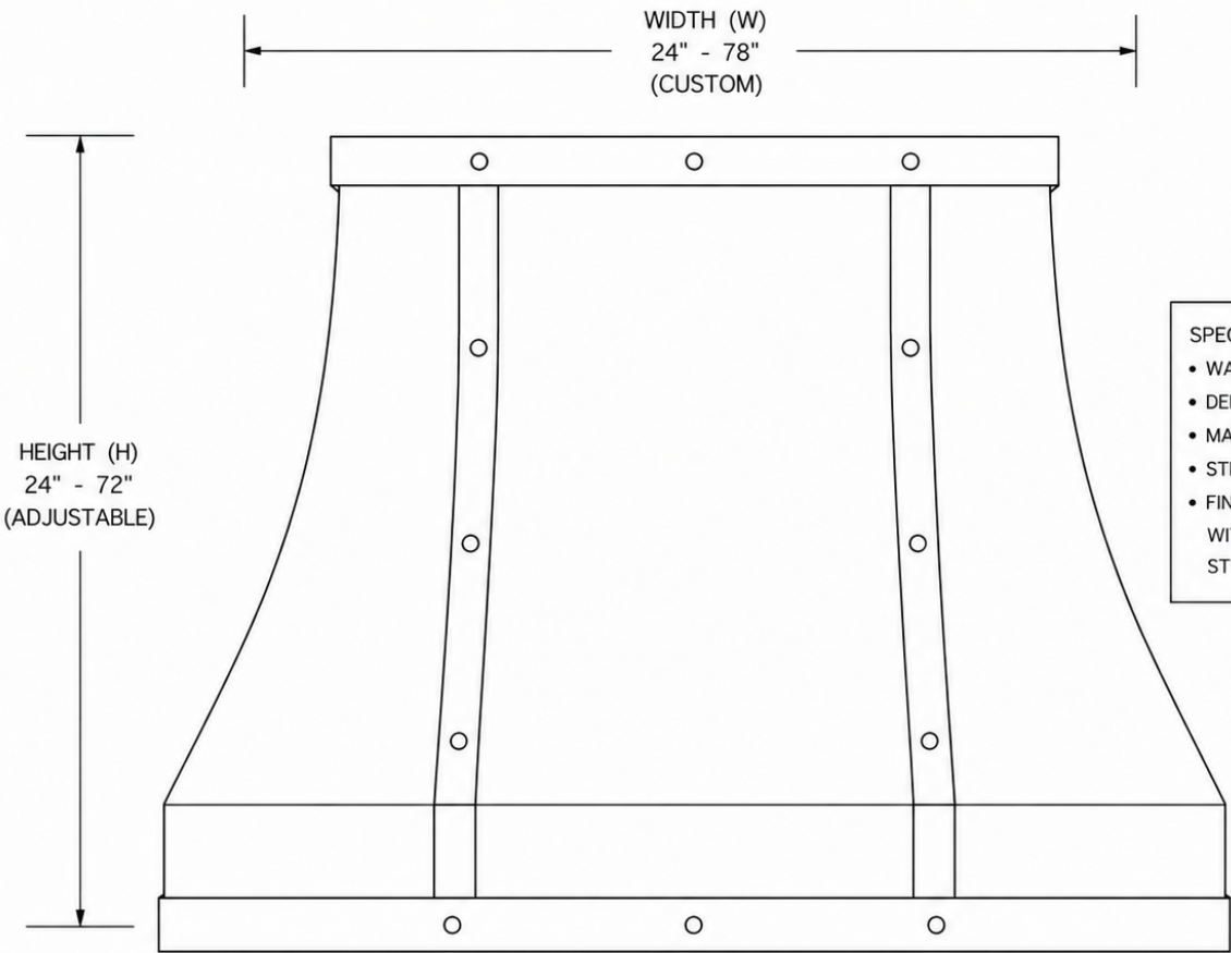
FRONT ELEVATION ALL DIMENSIONS ARE NOMINAL
